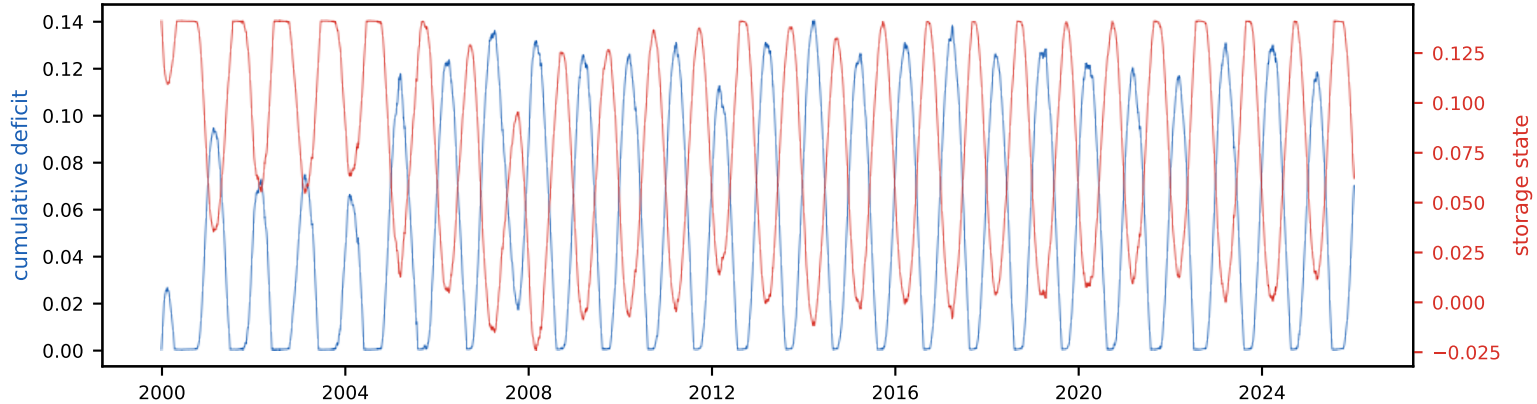
Cumulative deficit & storage state (peak deficit = required storage, S_{\text{tot}} =14.1% of annual)
