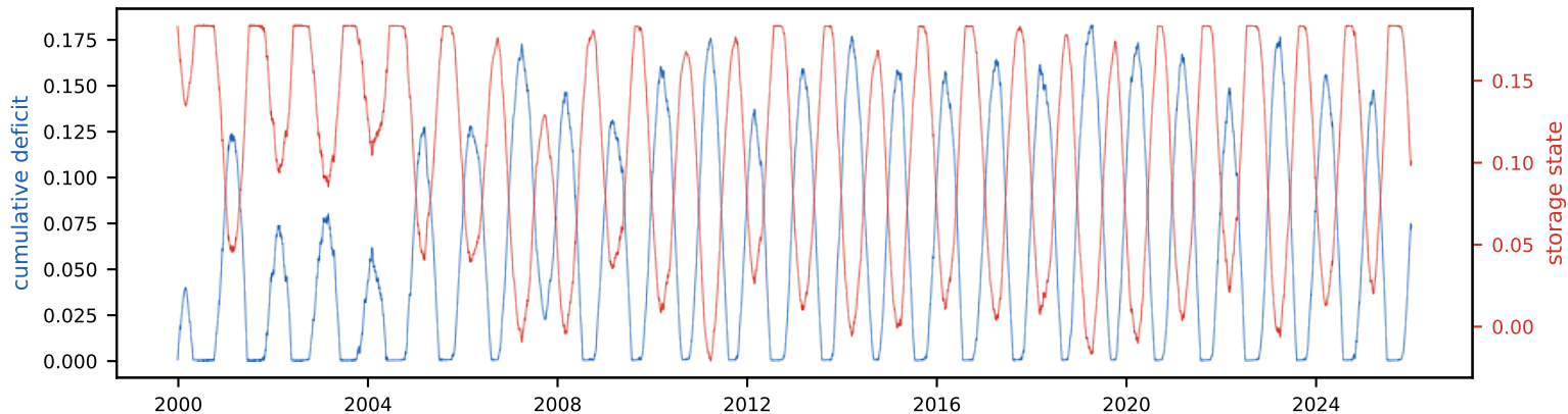
Cumulative deficit & storage state (peak deficit = required storage, S_{\text{tot}} =18.4% of annual)
