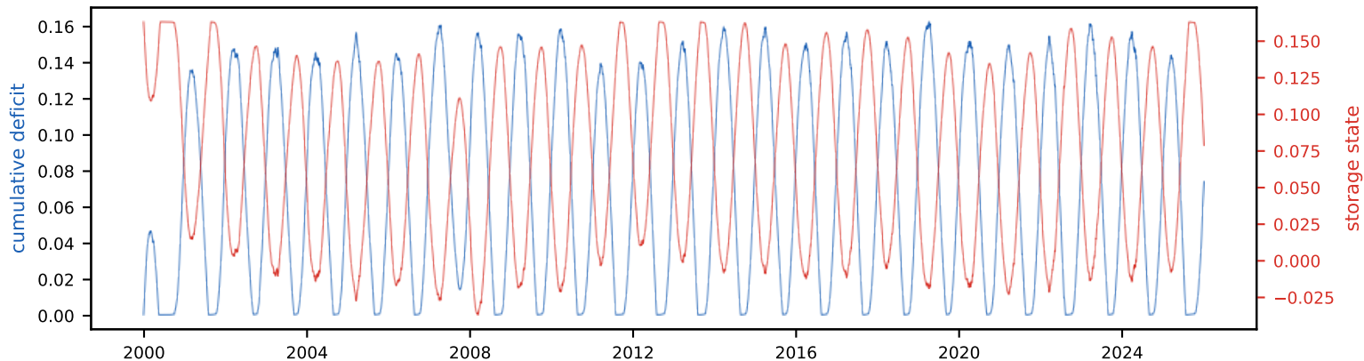
Cumulative deficit & storage state (peak deficit = required storage, S_{\text{tot}} =16.4% of annual)
