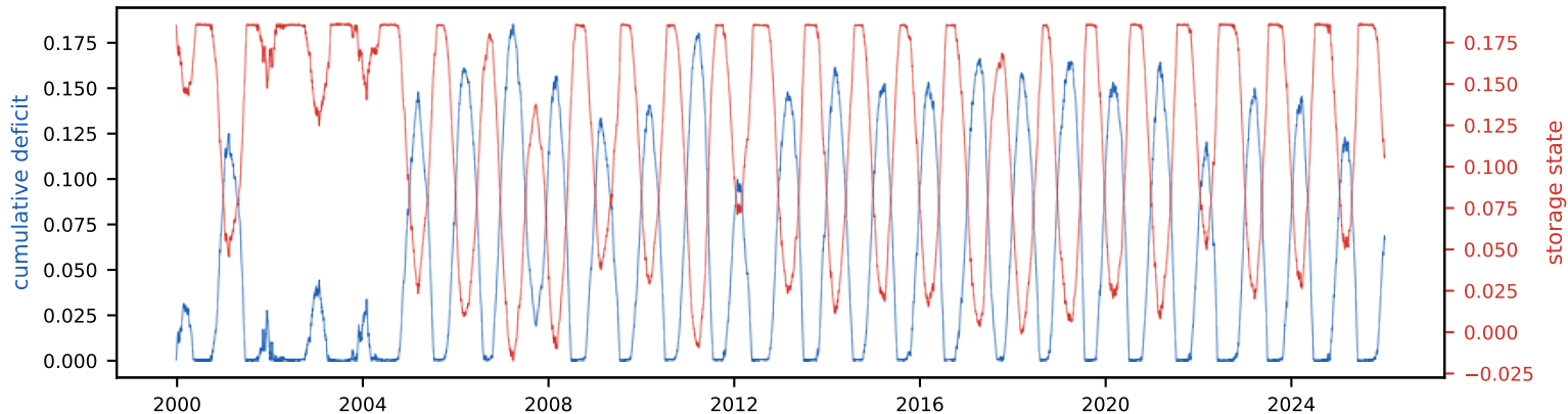
Cumulative deficit & storage state (peak deficit = required storage, S_{\text{tot}} =18.6% of annual)
