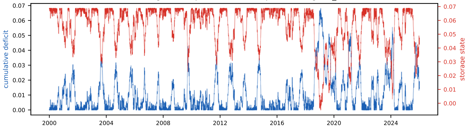
Real energy vs EIA demand (69 TWh/yr, 0.4% land)
