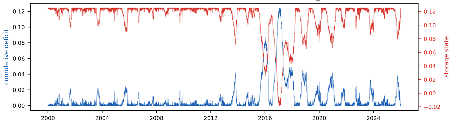
Real energy vs EIA demand (82 TWh/yr, 1.4% land)
