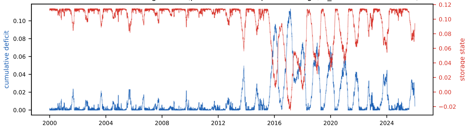
Real energy vs EIA demand (100 TWh/yr, 1.8% land)
