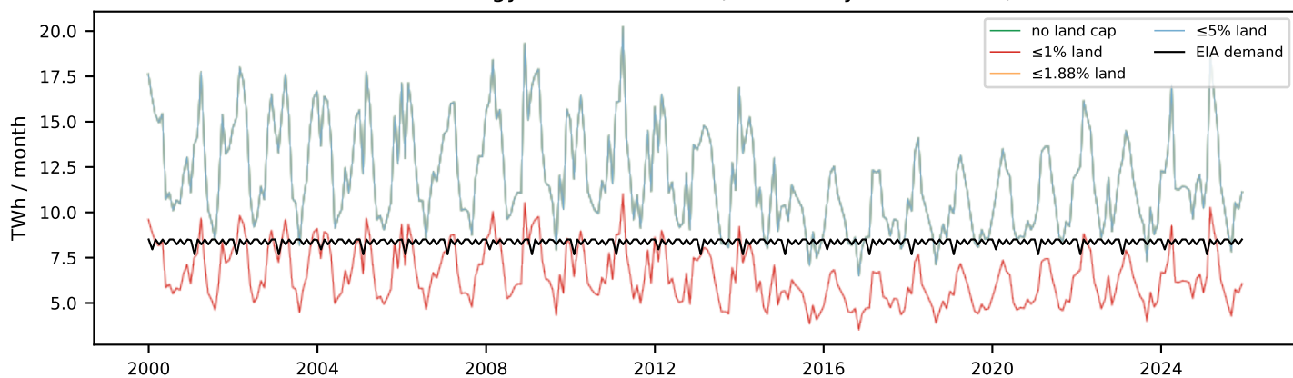
Real energy vs EIA demand (100 TWh/yr, 1.8% land)
