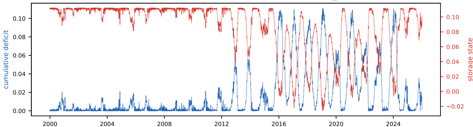
Real energy vs EIA demand (32 TWh/yr, 1.0% land)
