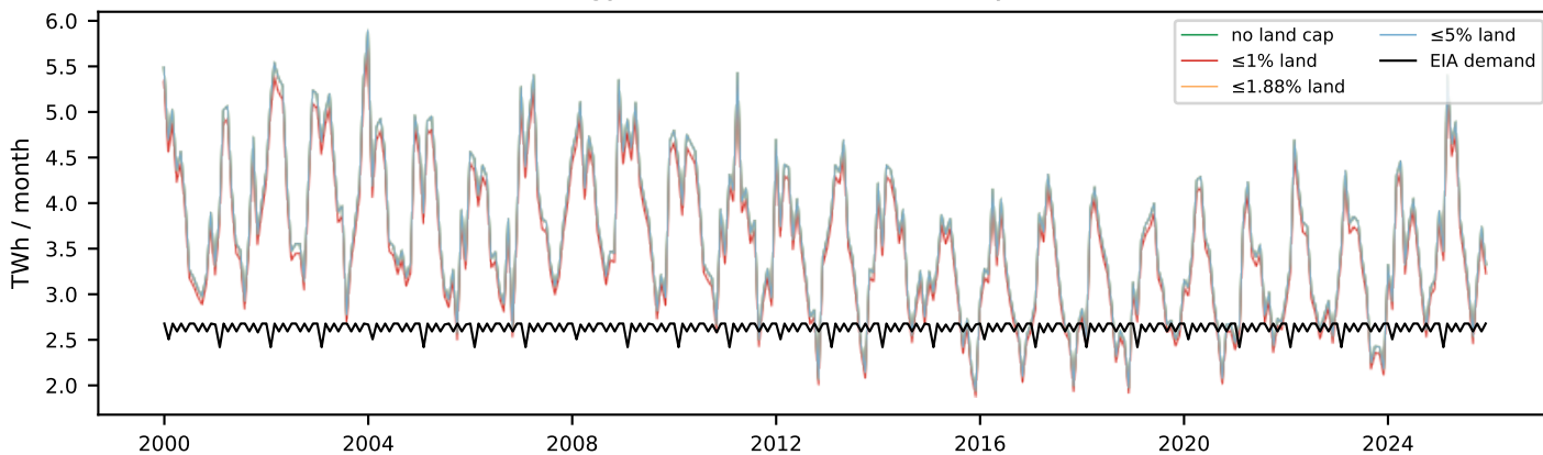
Real energy vs EIA demand (32 TWh/yr, 1.0% land)
