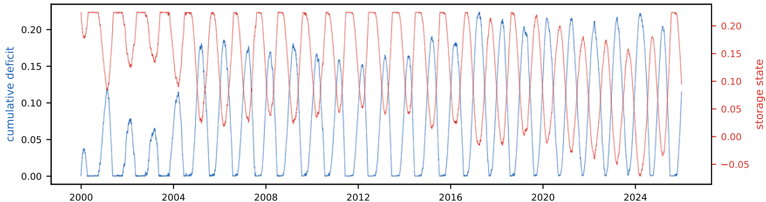
Cumulative deficit & storage state (peak deficit = required storage, S_{\text{tot}} =22.5% of annual)
