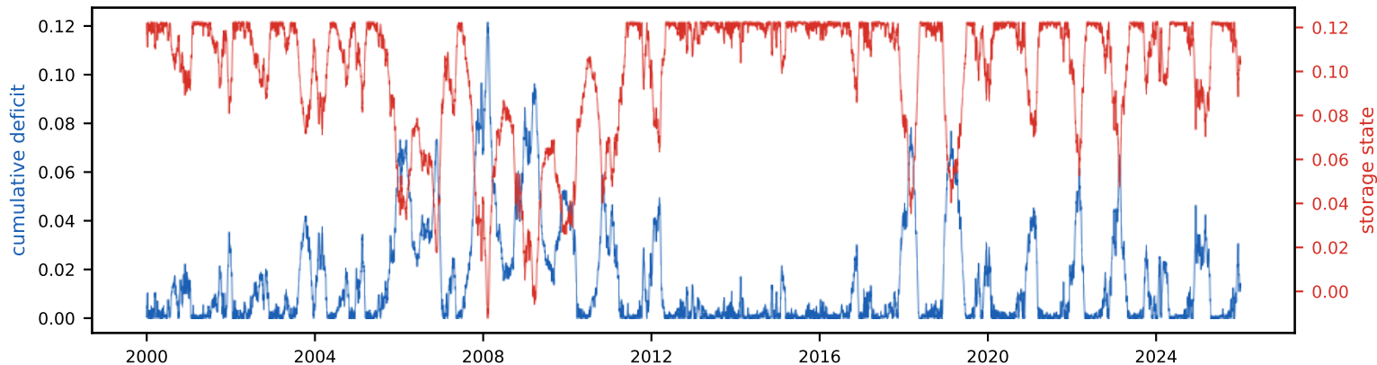
Cumulative deficit & storage state (peak deficit = required storage, S_{tot} =12.2% of annual)
