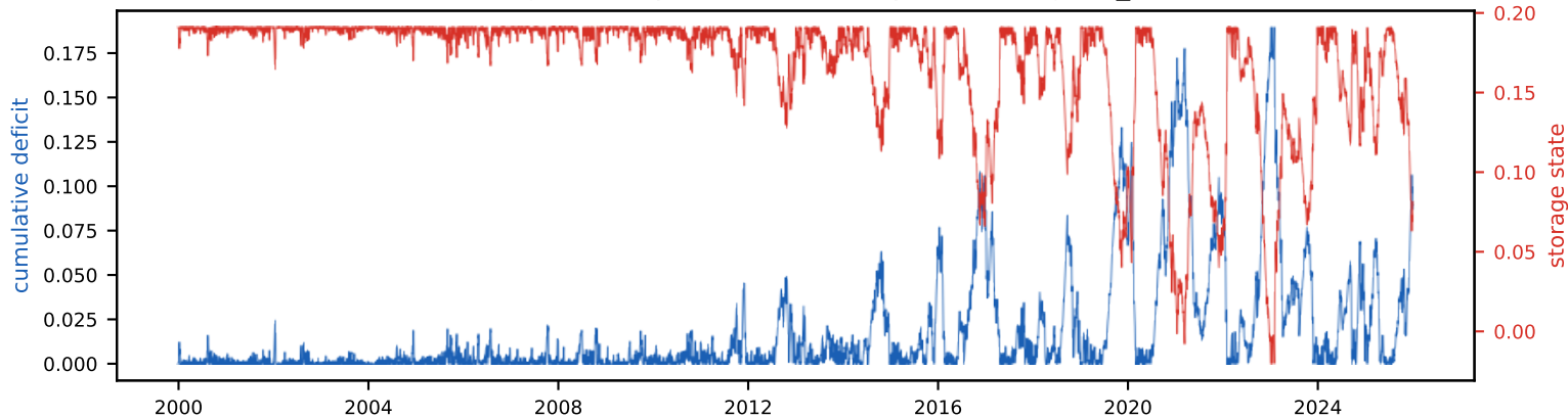
Cumulative deficit & storage state (peak deficit = required storage, S_{\text{tot}} =19.1% of annual)
