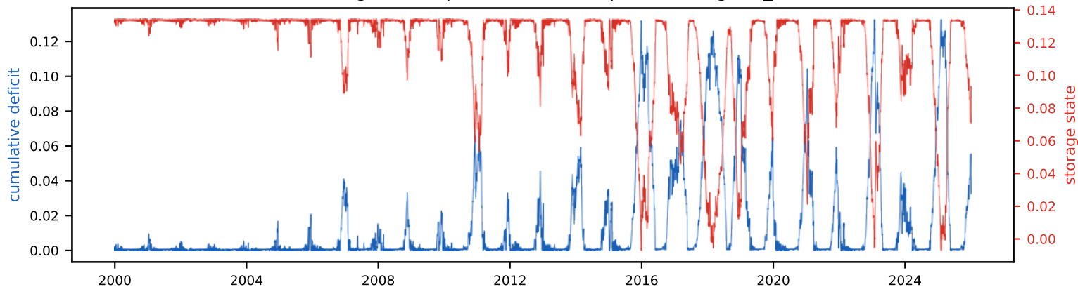
Cumulative deficit & storage state (peak deficit = required storage, S_{\text{tot}} =13.4% of annual)
