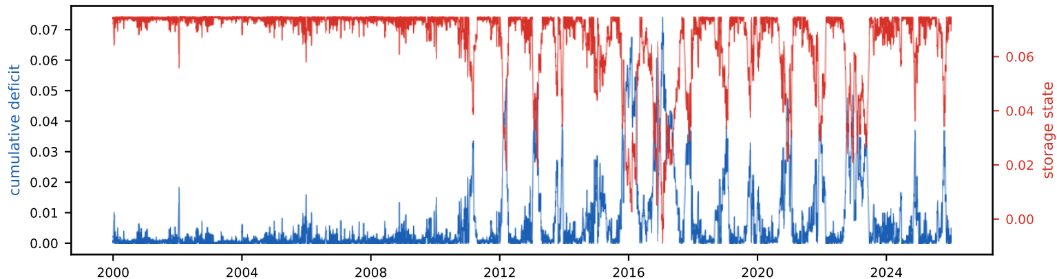
Cumulative deficit & storage state (peak deficit = required storage, S_{\text{tot}} =7.5% of annual)
