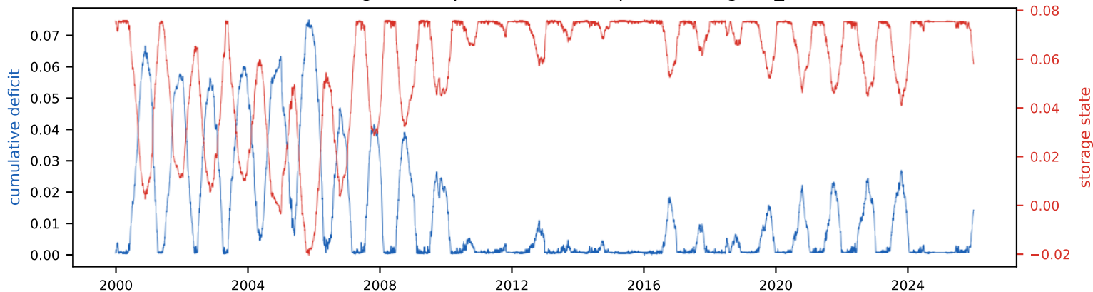
Cumulative deficit & storage state (peak deficit = required storage, S_{\text{tot}} =7.6% of annual)
