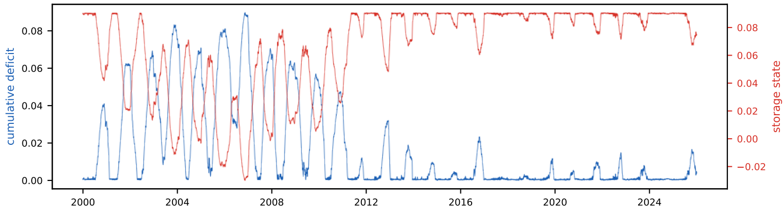
Cumulative deficit & storage state (peak deficit = required storage, S_{tot}=9.1\% of annual)
