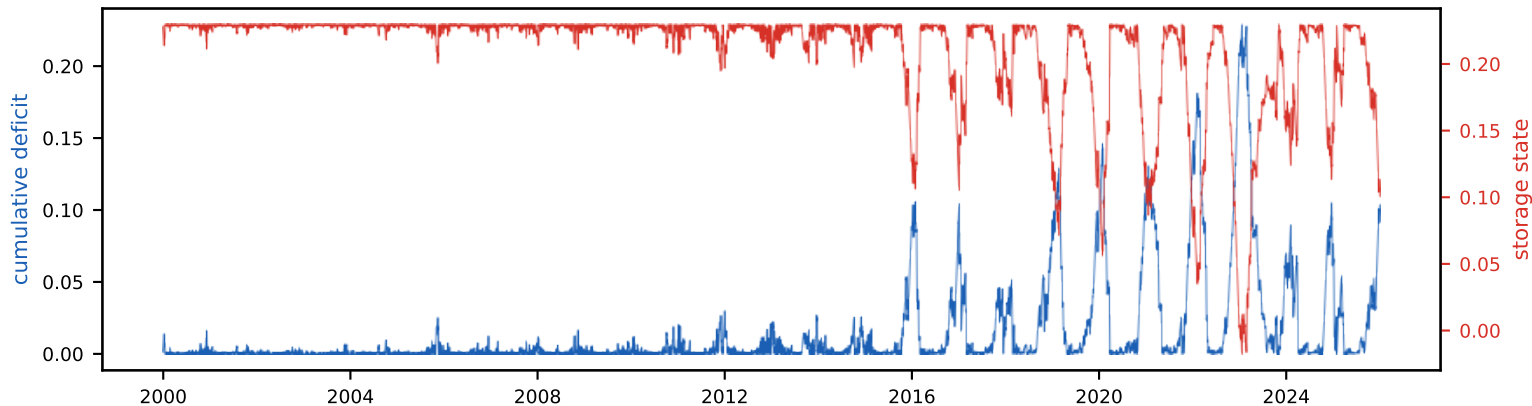
Cumulative deficit & storage state (peak deficit = required storage, S_{\text{tot}} =22.9% of annual)
