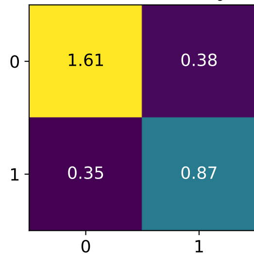
Transformed \tilde{f}_0
