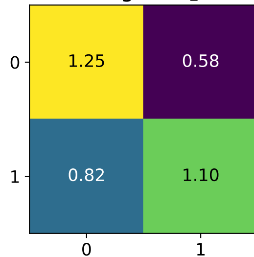
Original f_2
