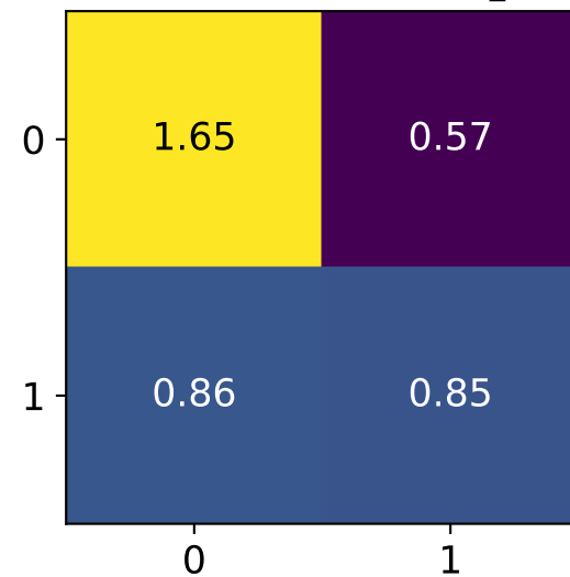
Transformed \tilde{f}_2
