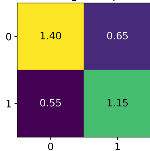
Original f_0
