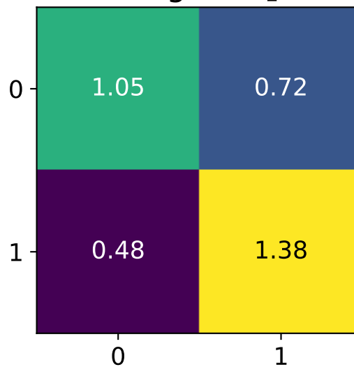
Original f_1
