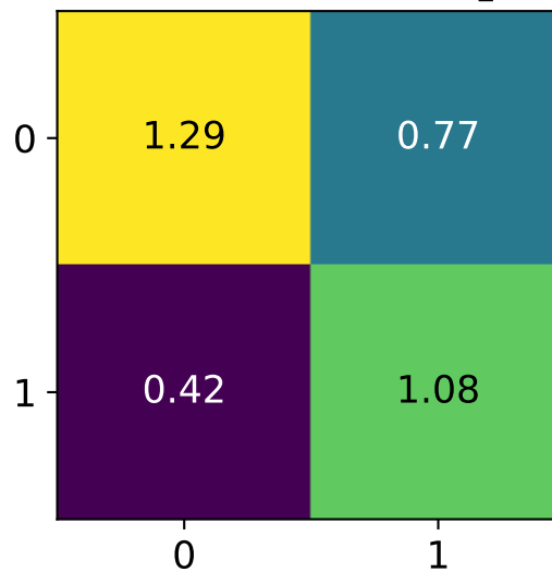
Transformed \tilde{f}_1
