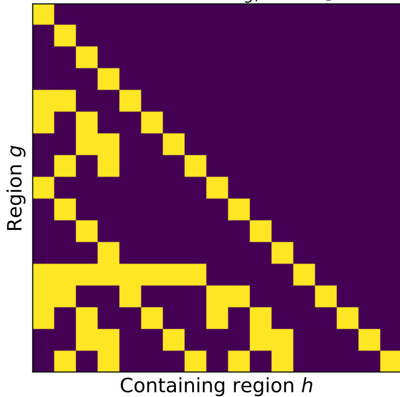
Inclusion matrix A_{g,h} = \mathbf{1}(g \subseteq h)
