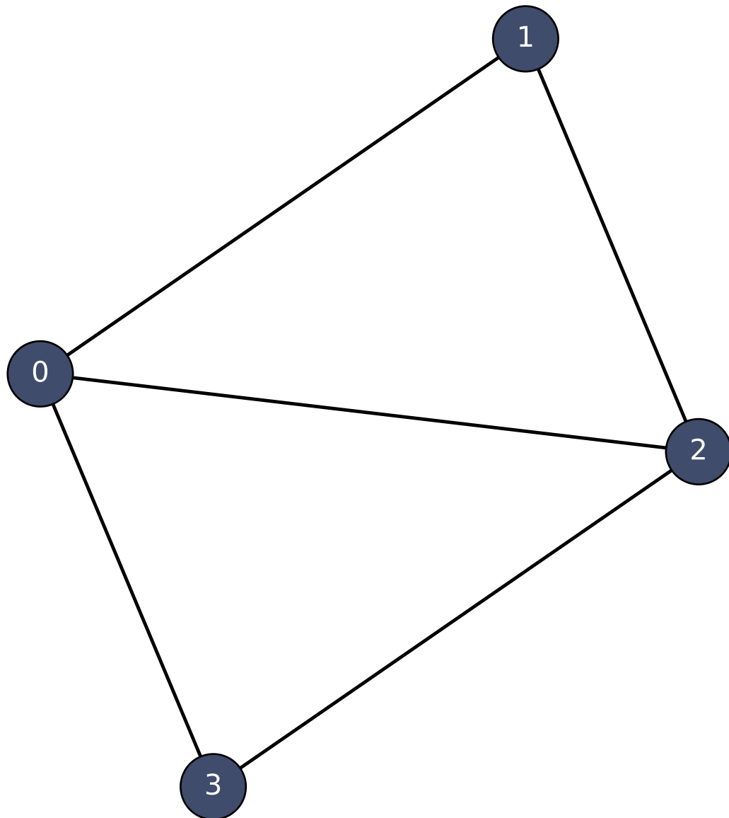
Original loopy graph
