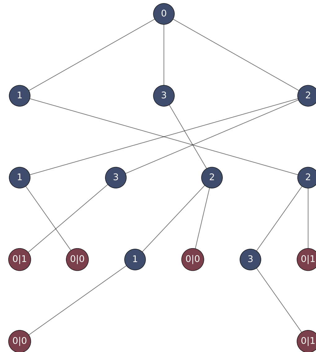
Self-avoiding-walk tree; v|0 and v|1 are pinned leaves
