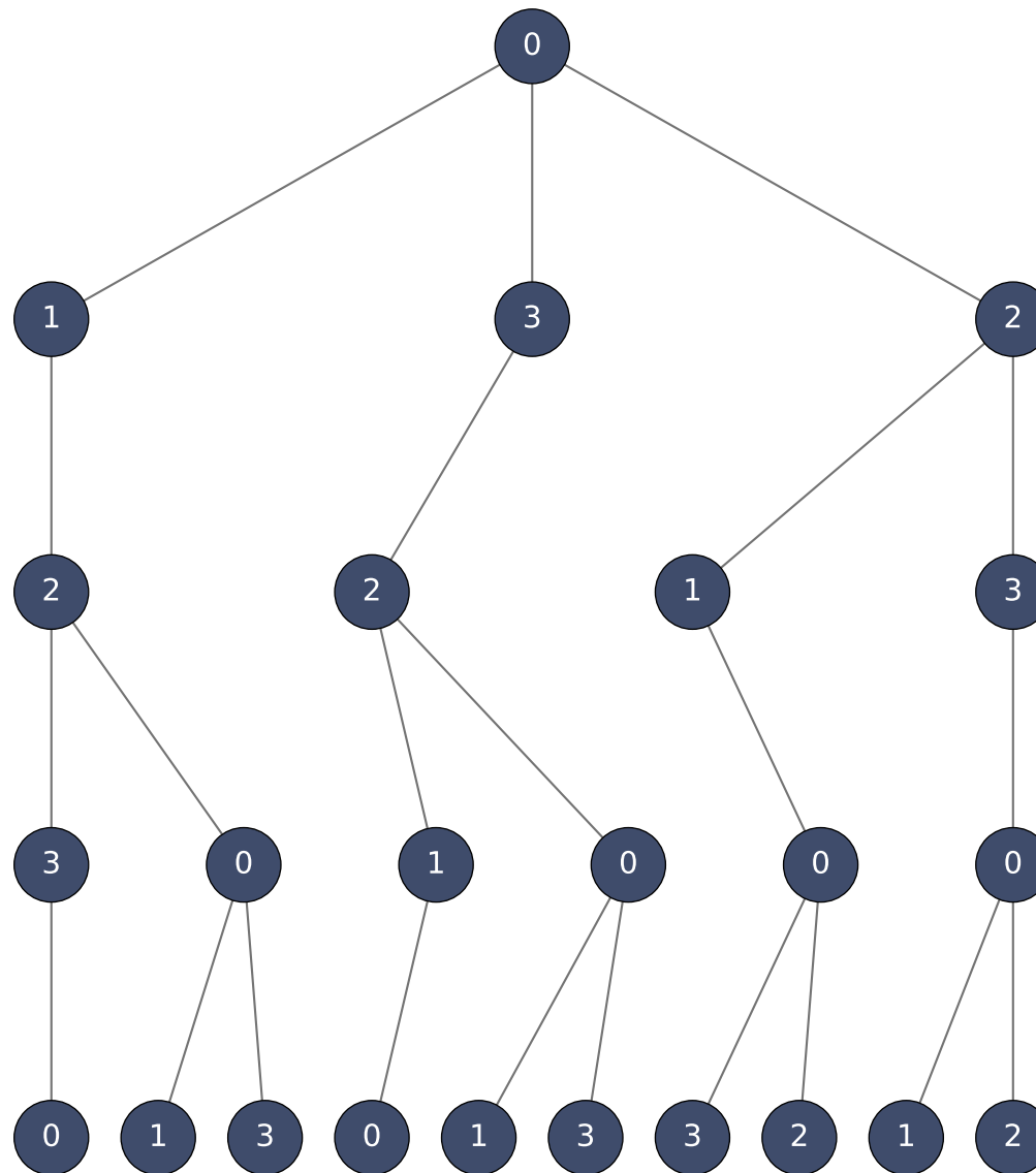
Computational tree, depth 4
