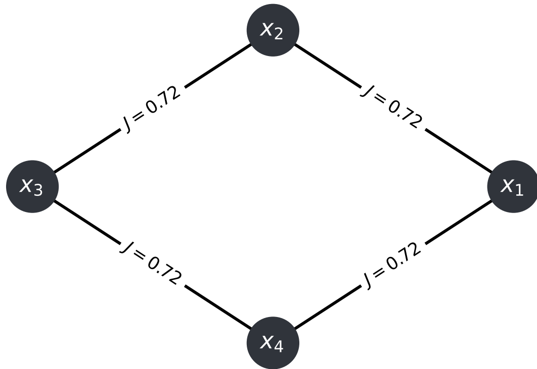
Four-spin cycle
