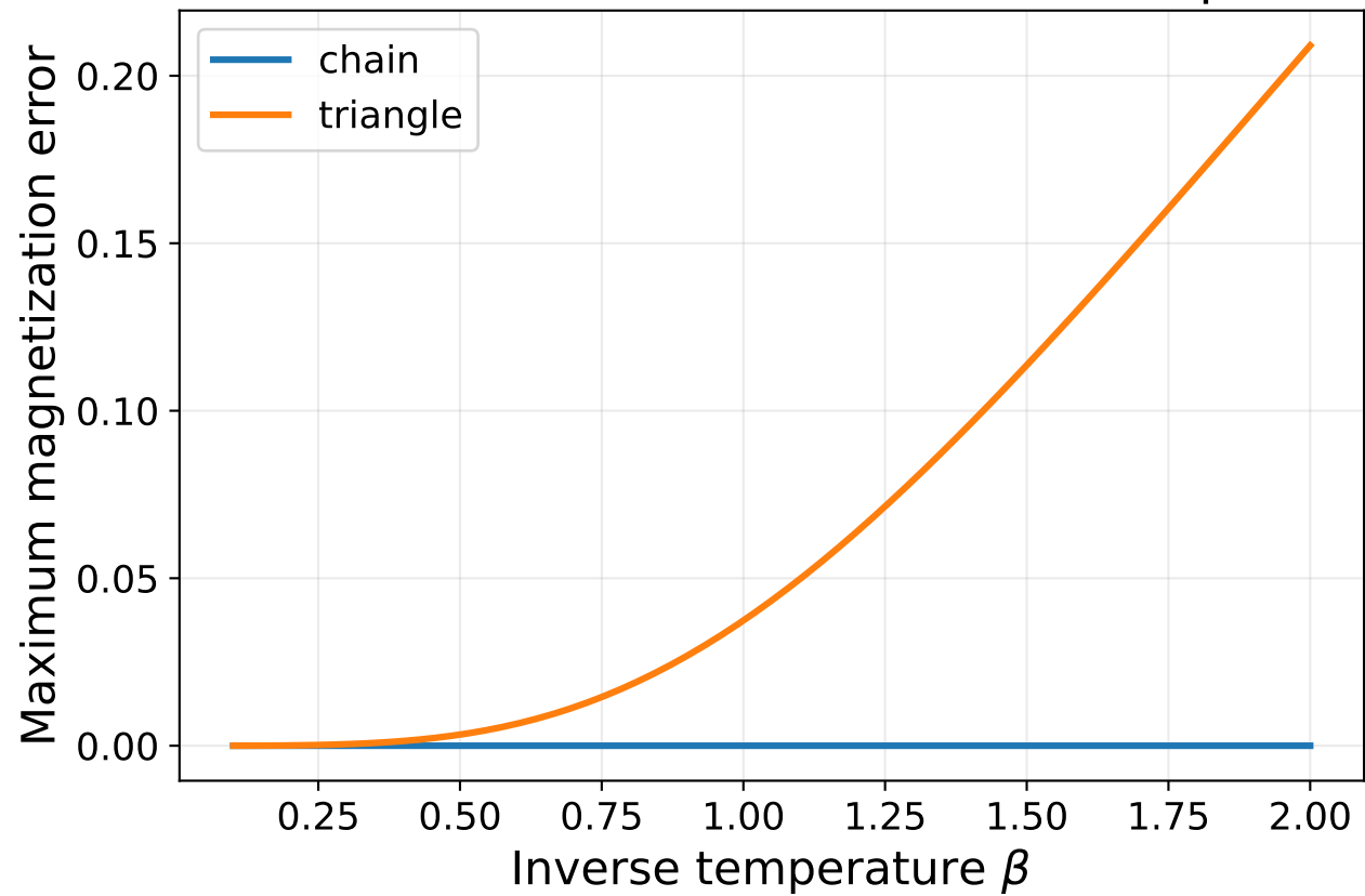
Bethe is exact on the chain but not on the loop Local beliefs inherit the same tree-versus-loop distinction
