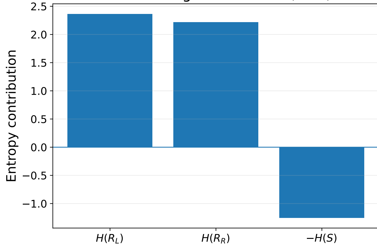
Kikuchi counting numbers: +1, +1, -1
