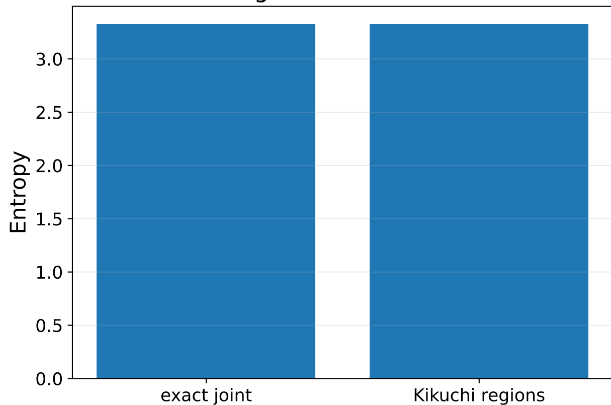
Exact agreement: H = 3.3273
