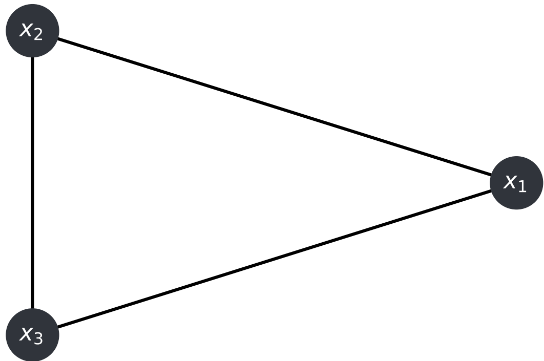
Frustrated antiferromagnetic triangle
