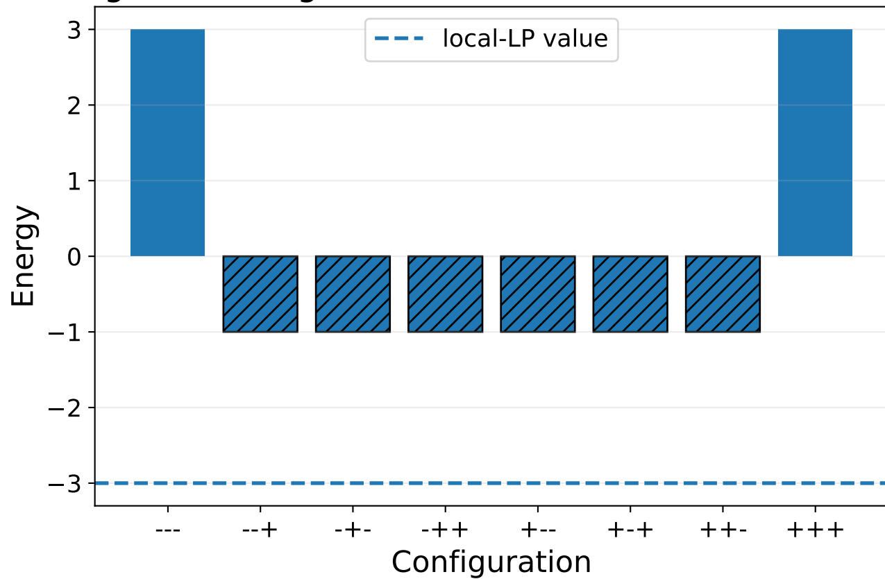
No global configuration realizes all three local wishes
