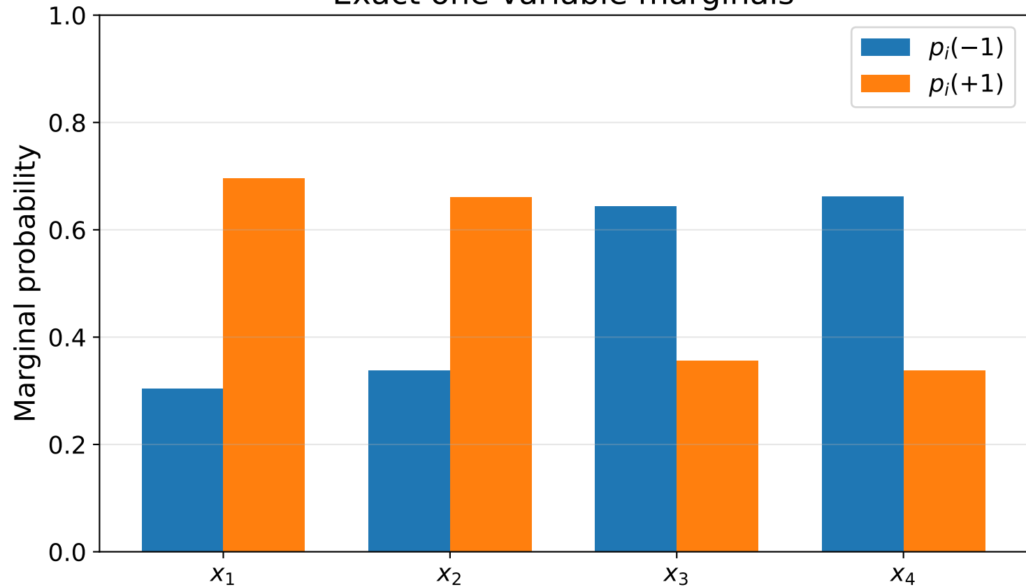
Exact one-variable marginals
