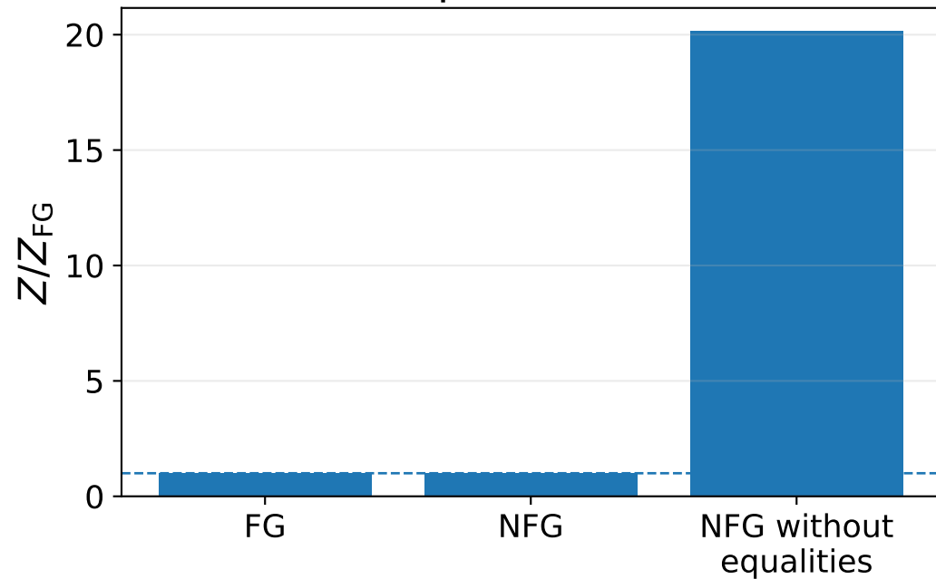
Relative partition function
