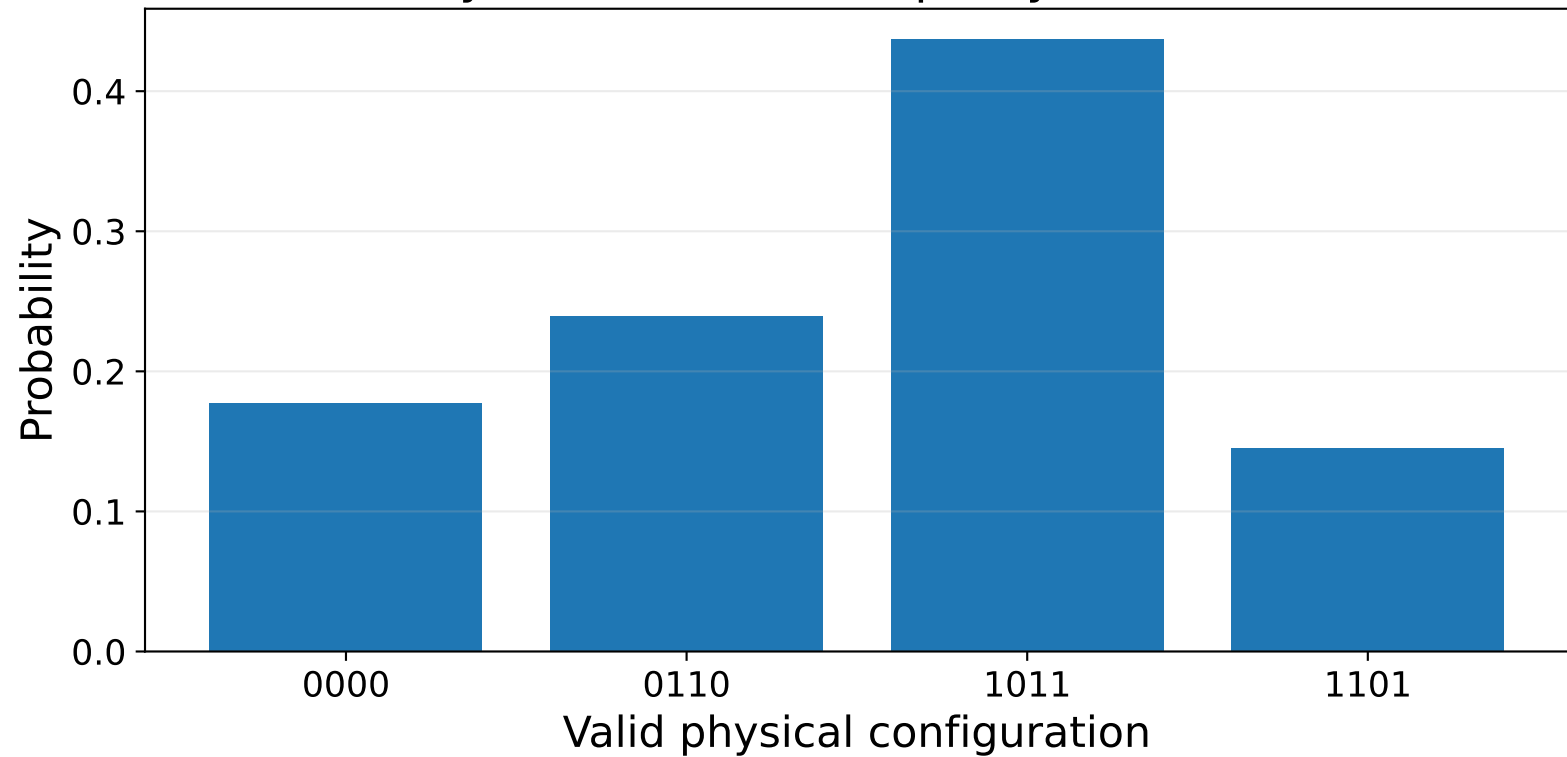
Probability distribution over parity-consistent states
