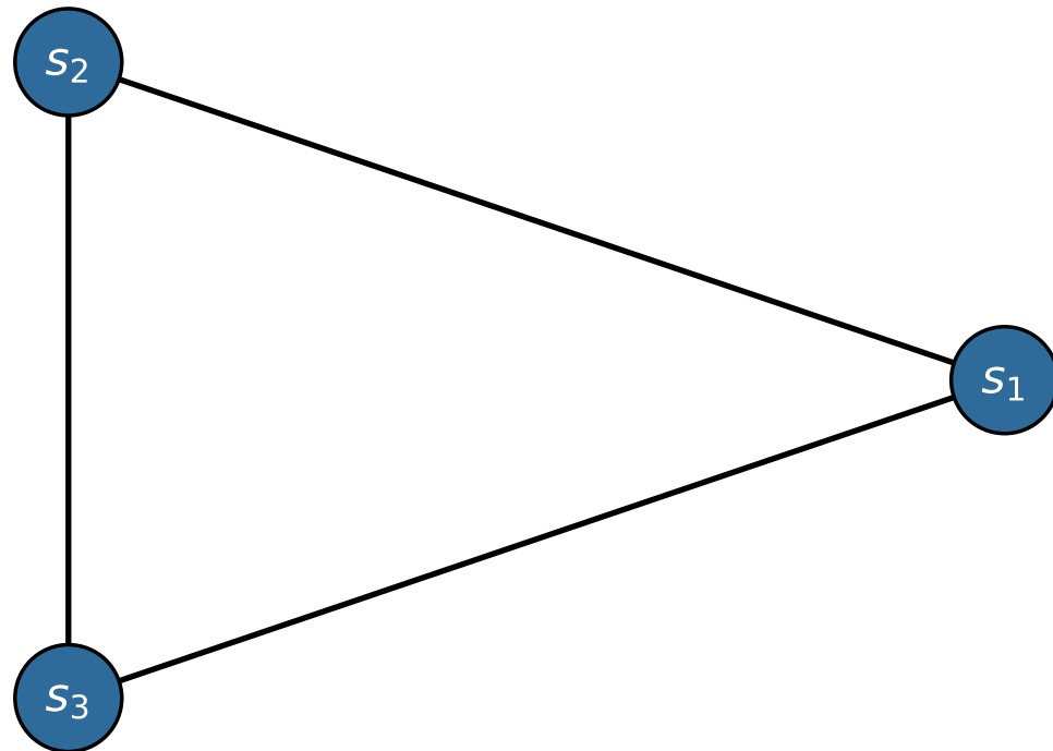
Three-spin triangle: one loop
