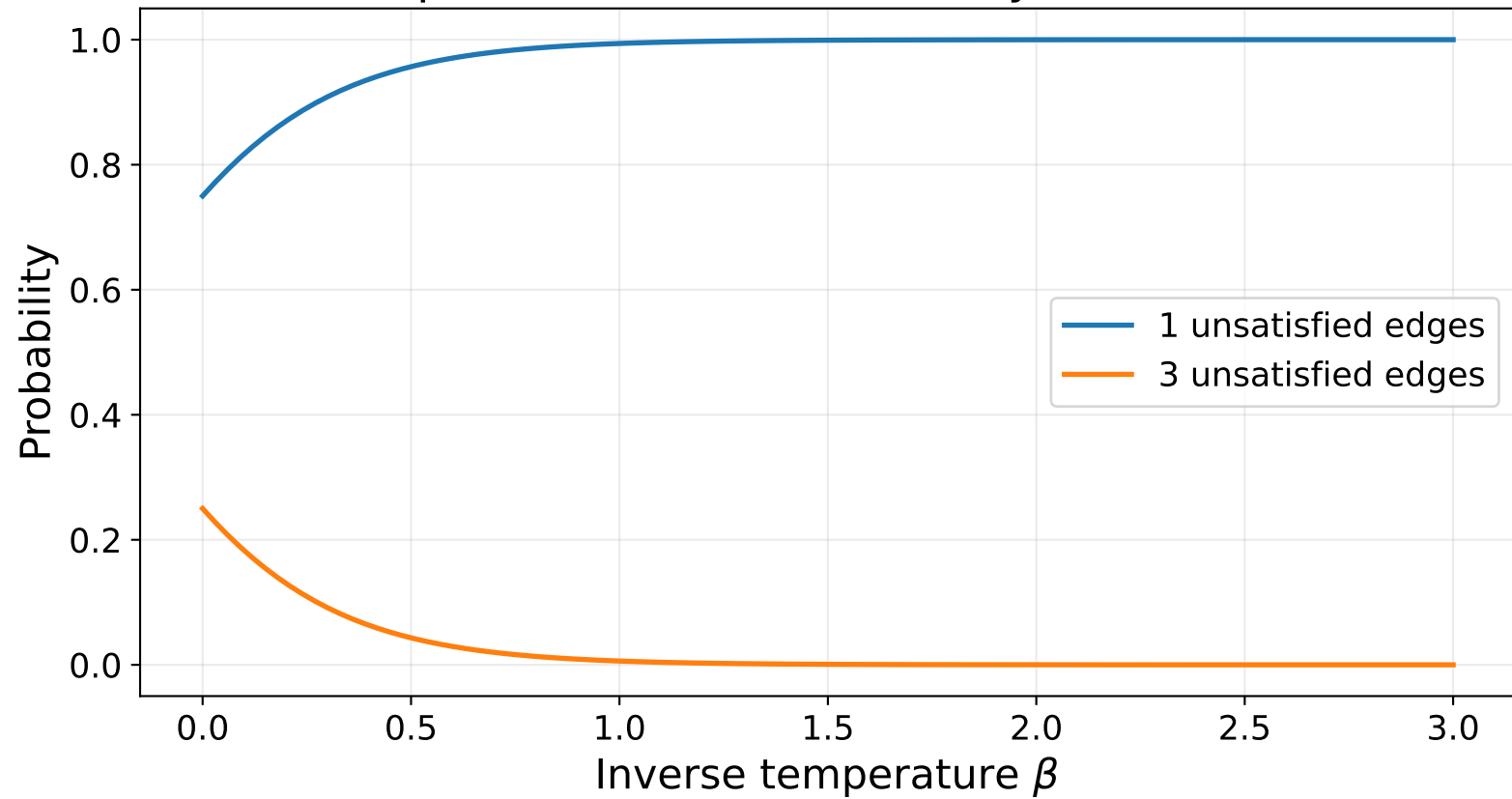
Low temperature selects minimally frustrated states
