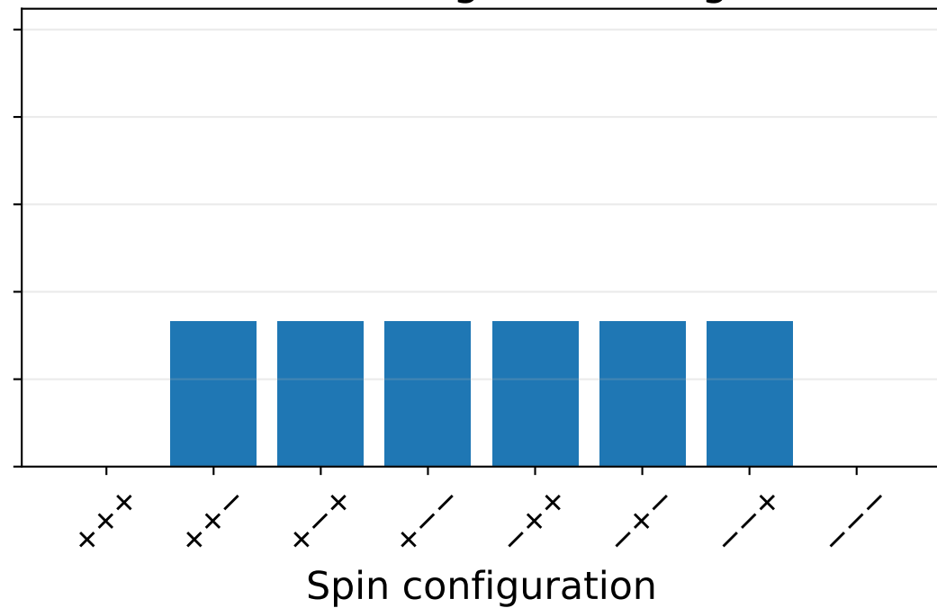
Antiferromagnetic triangle
