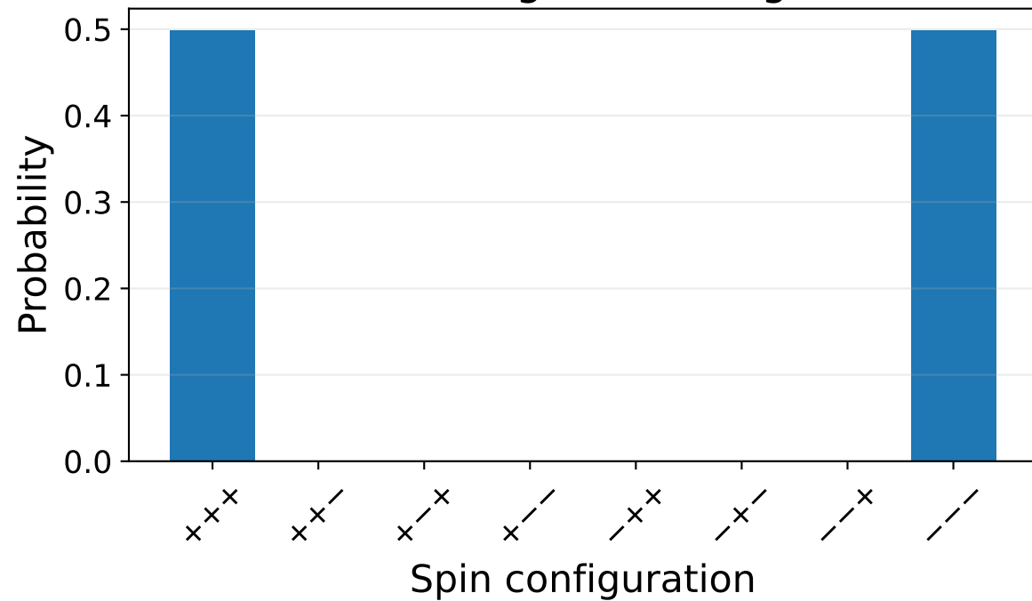
Ferromagnetic triangle
