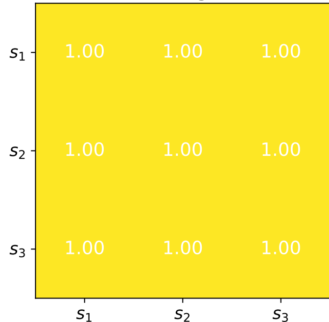
Ferromagnetic
