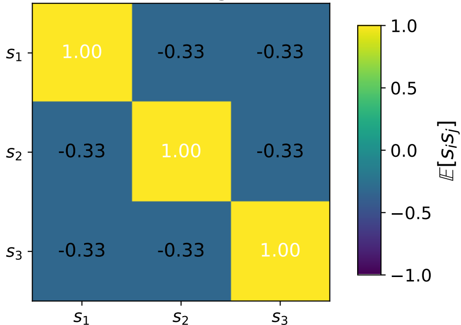
Antiferromagnetic
