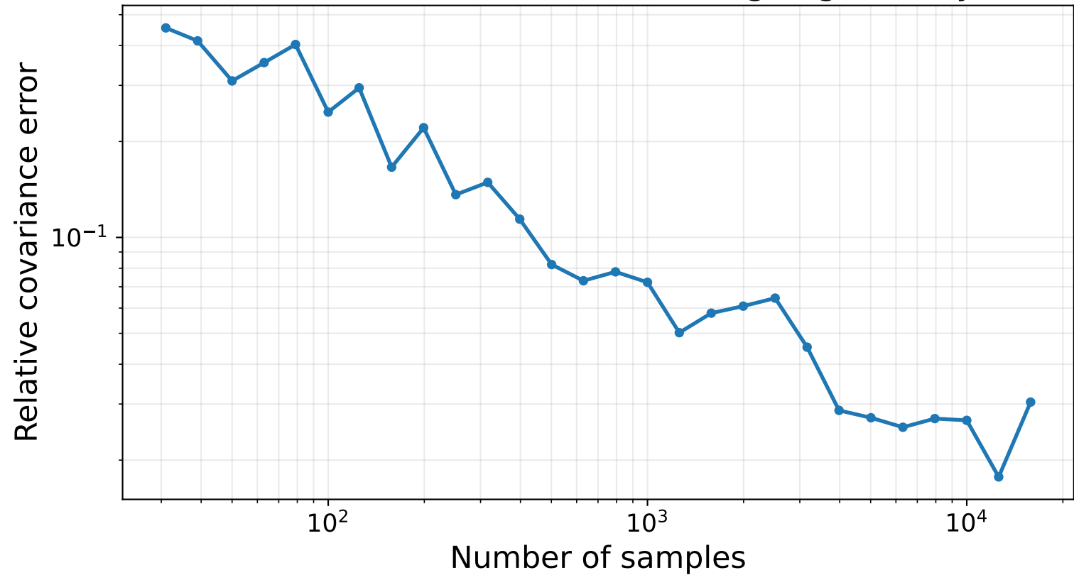
Monte Carlo estimation converges gradually
