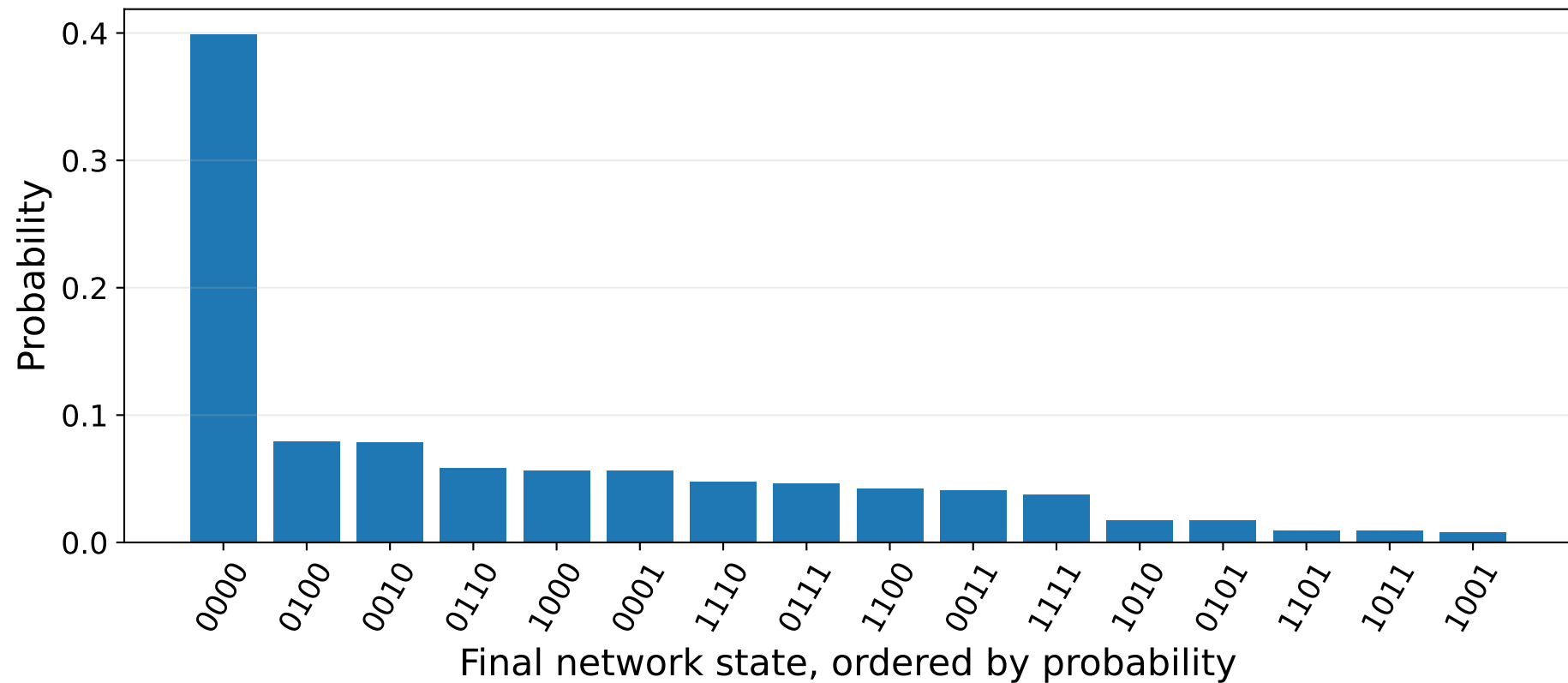
Exact state distribution at time T = 9
