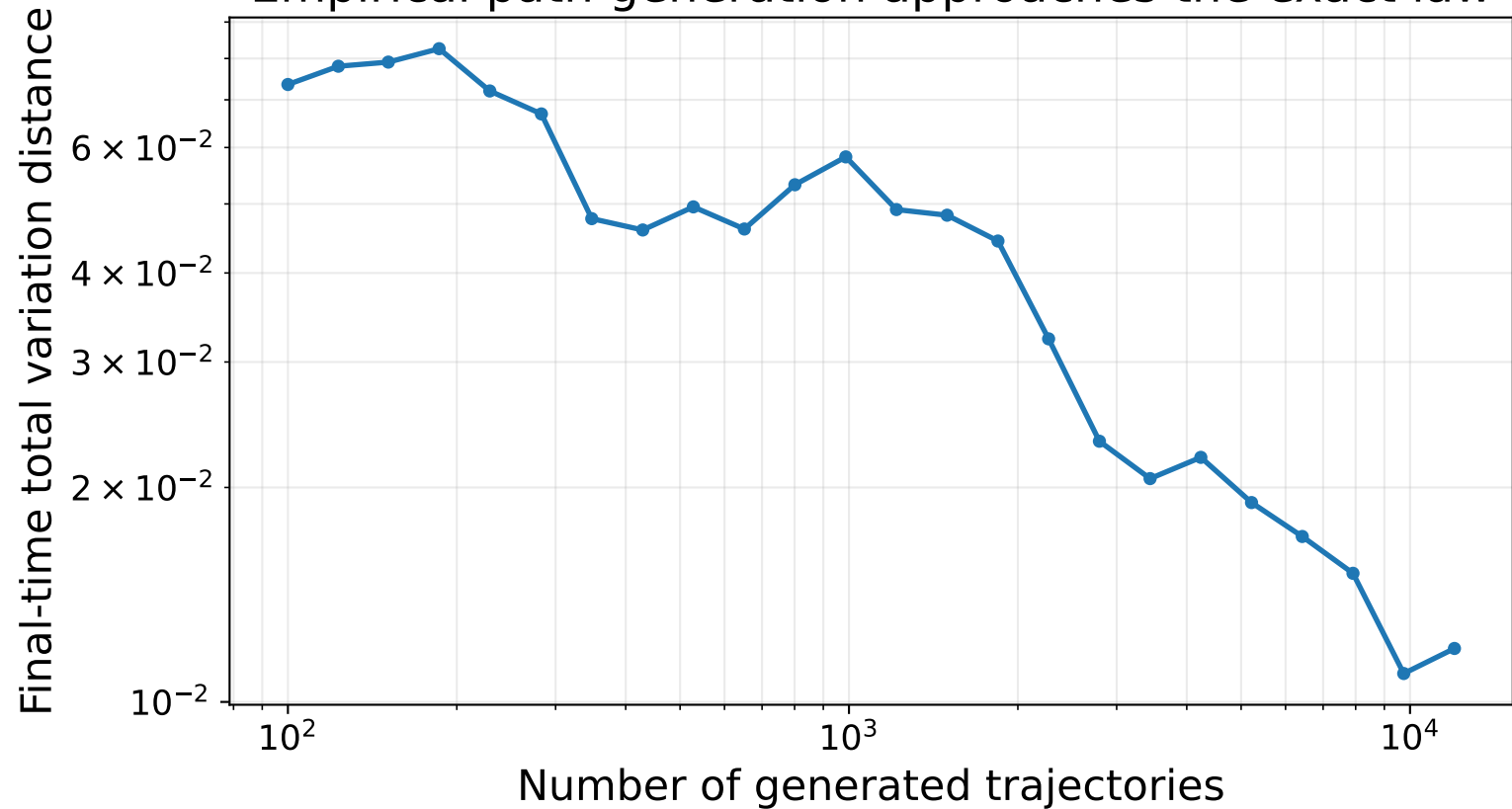
Empirical path generation approaches the exact law
