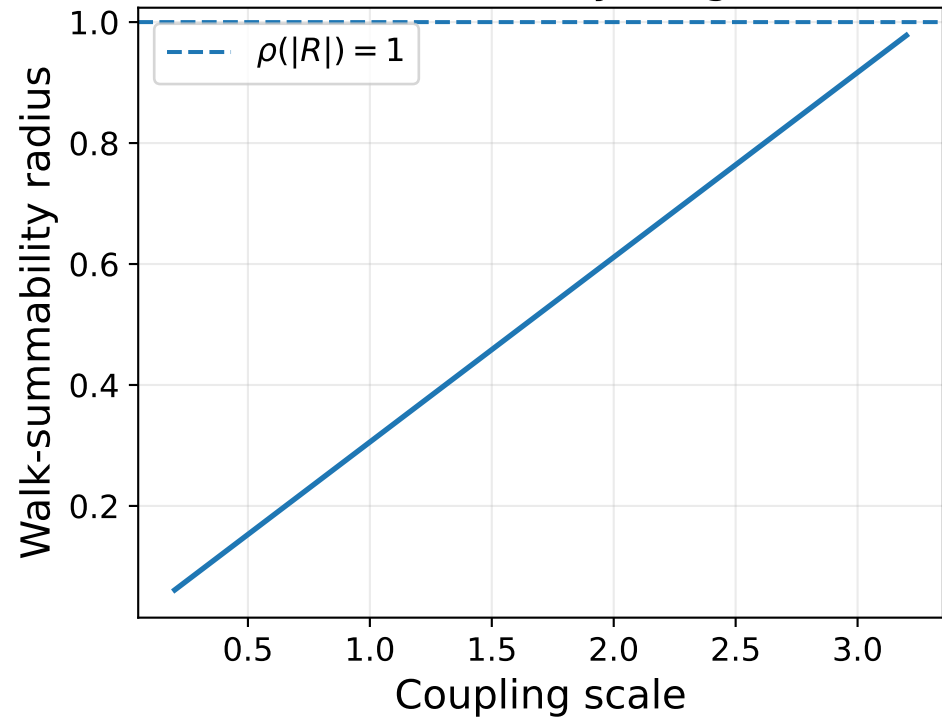
Walk-summability diagnostic
