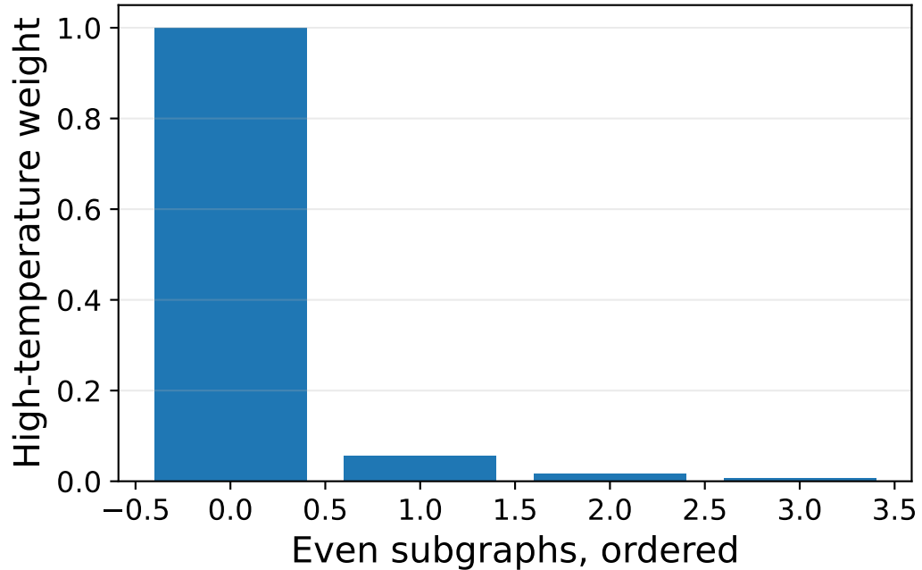
4 even subgraphs contribute
