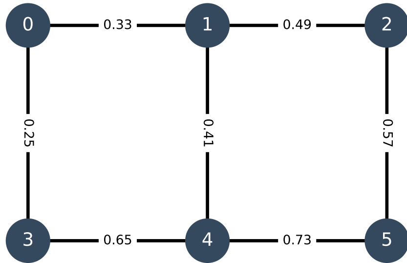
Planar zero-field Ising graph
