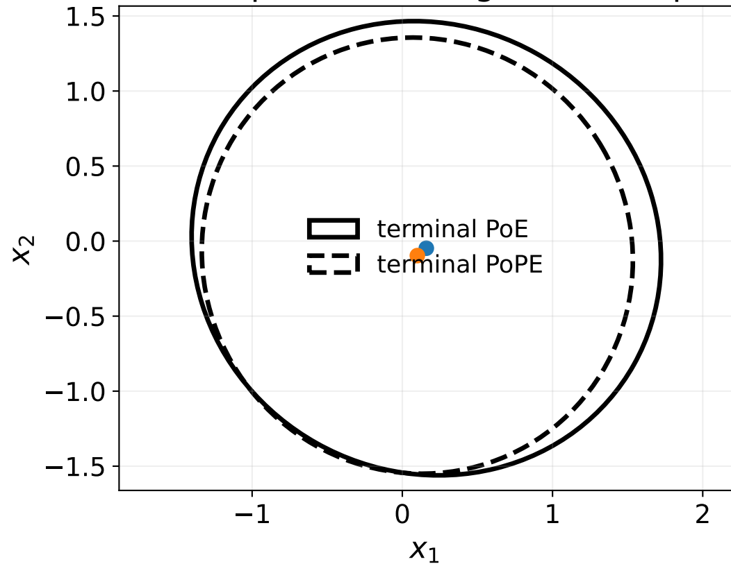
Path composition changes the endpoint
