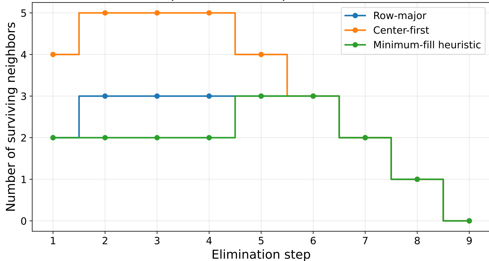
Intermediate separator sizes depend on elimination order
