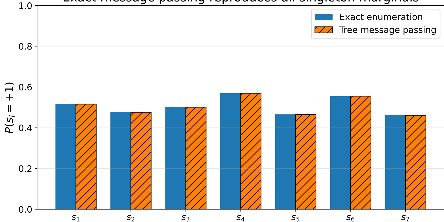
Exact message passing reproduces all singleton marginals
