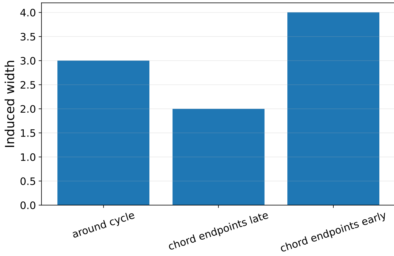
Elimination order controls exact cost
