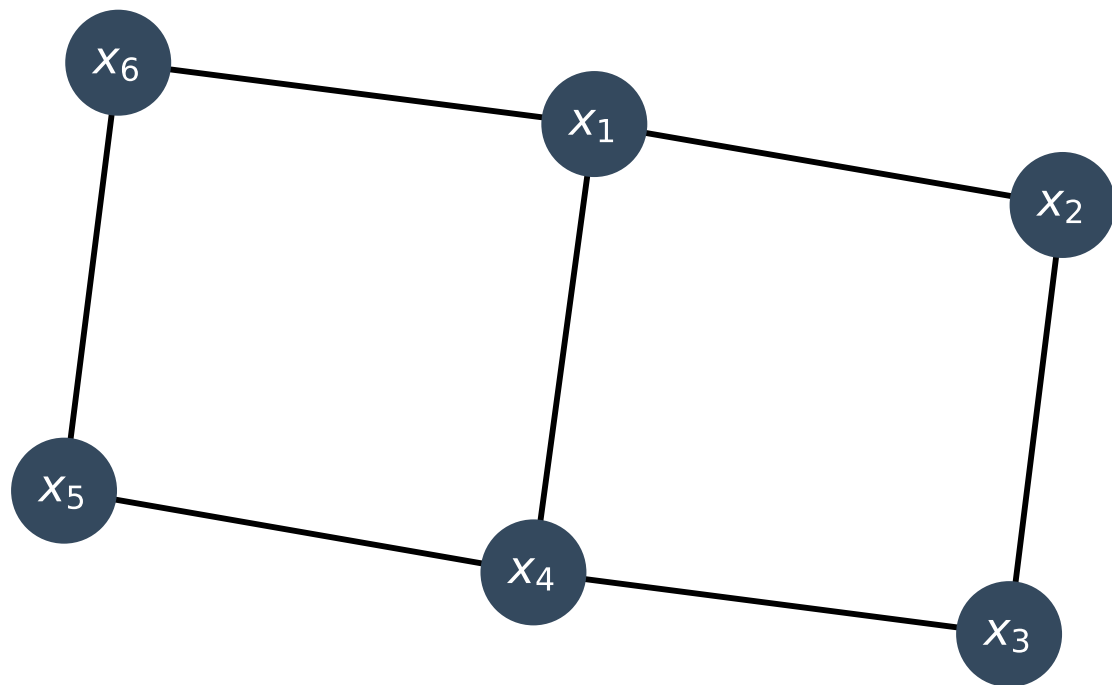
Interaction graph
