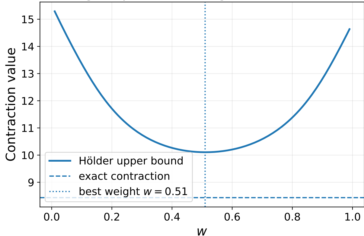
Weight optimization tightens the bound
