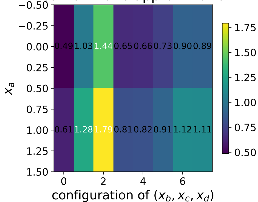
Best rank-one approximation
