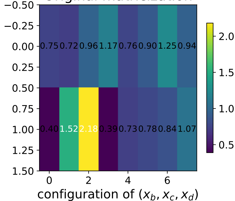
Original matricization
