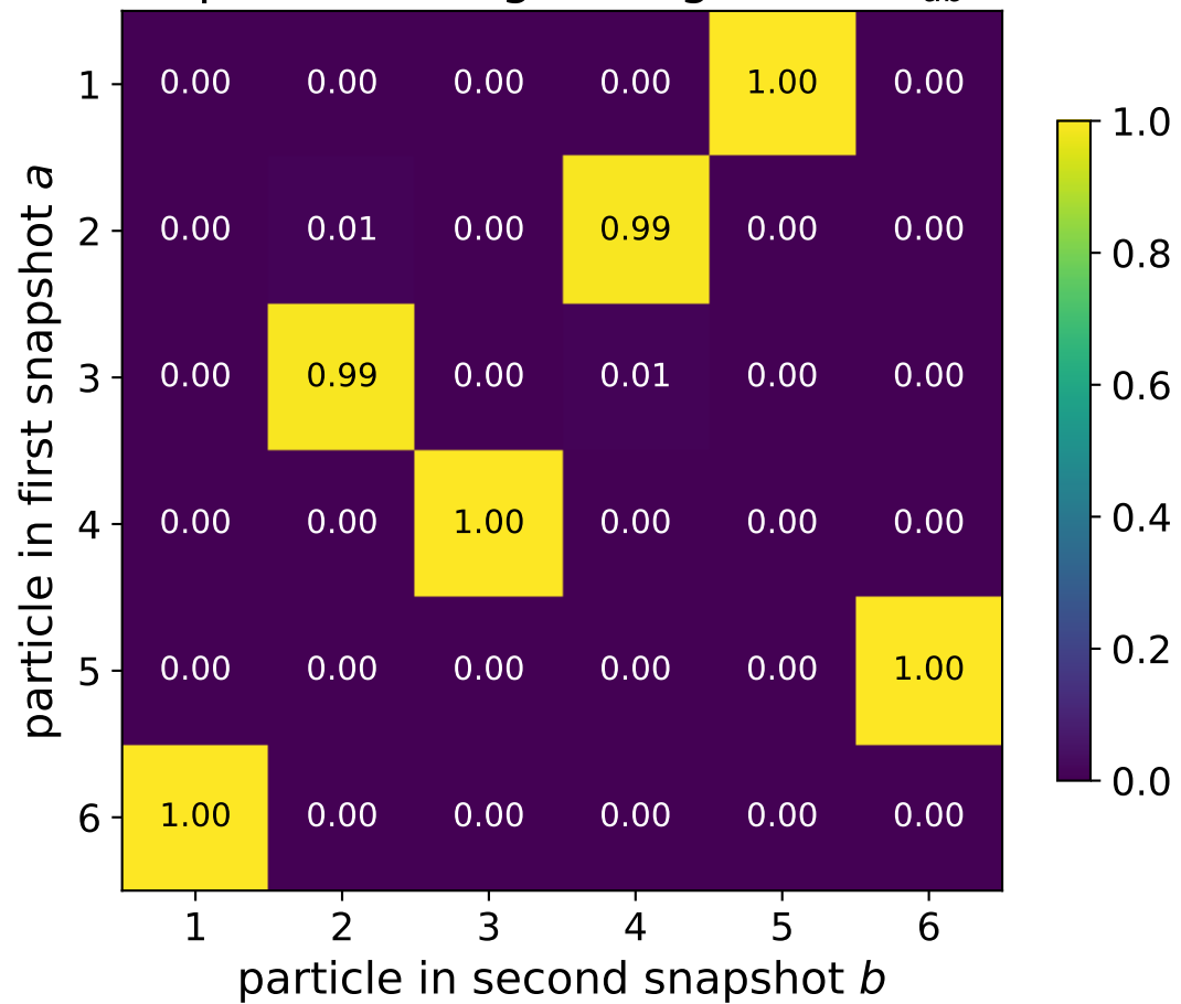
Exact posterior edge marginals P(x_{ab} = 1)
