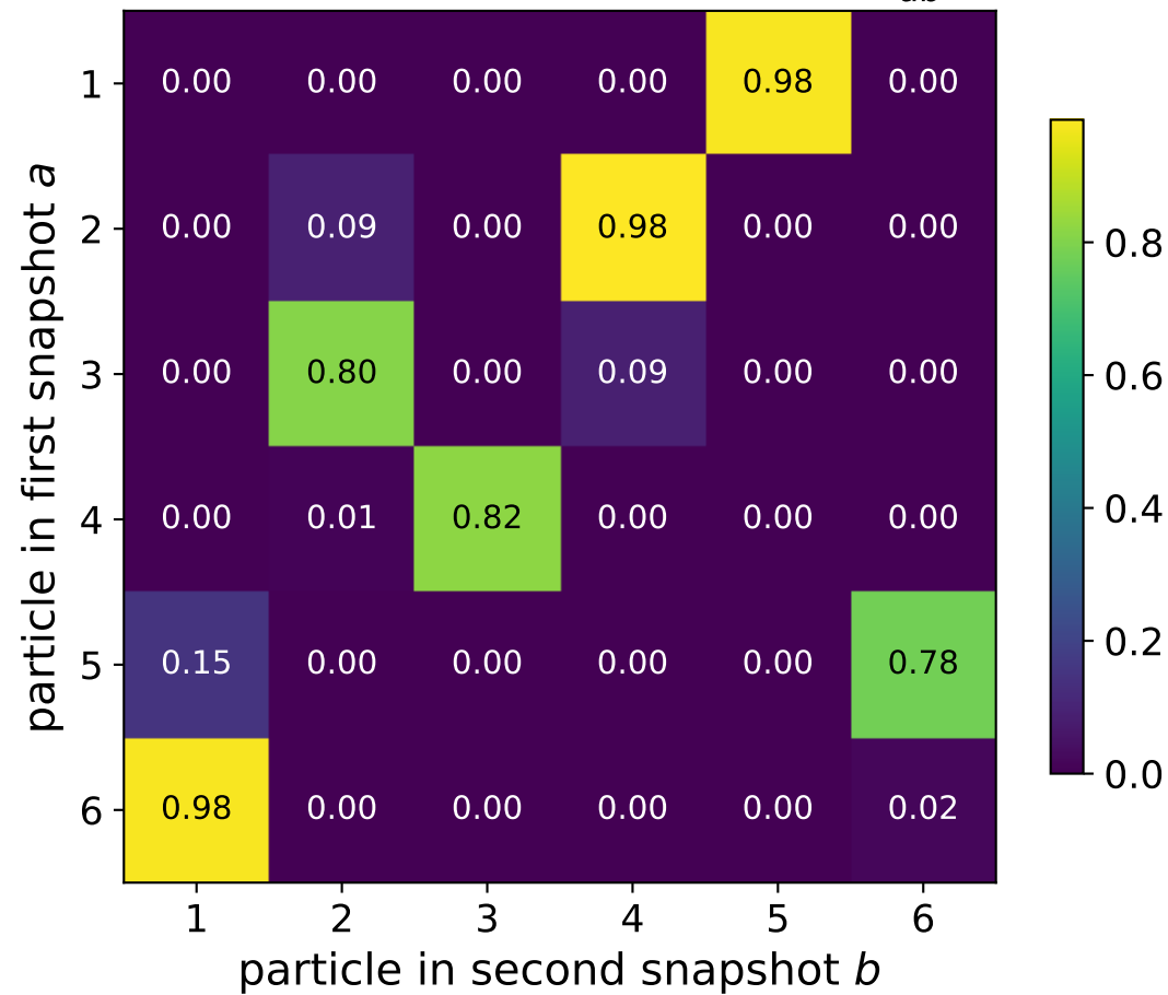
Local transition likelihoods W_{ab}
