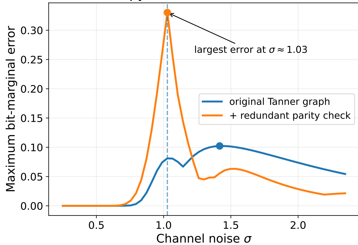
Loopy BP failure versus noise
