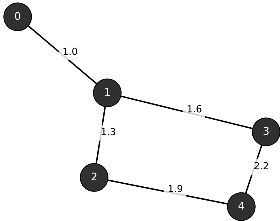
Physical network; edge labels are susceptances
