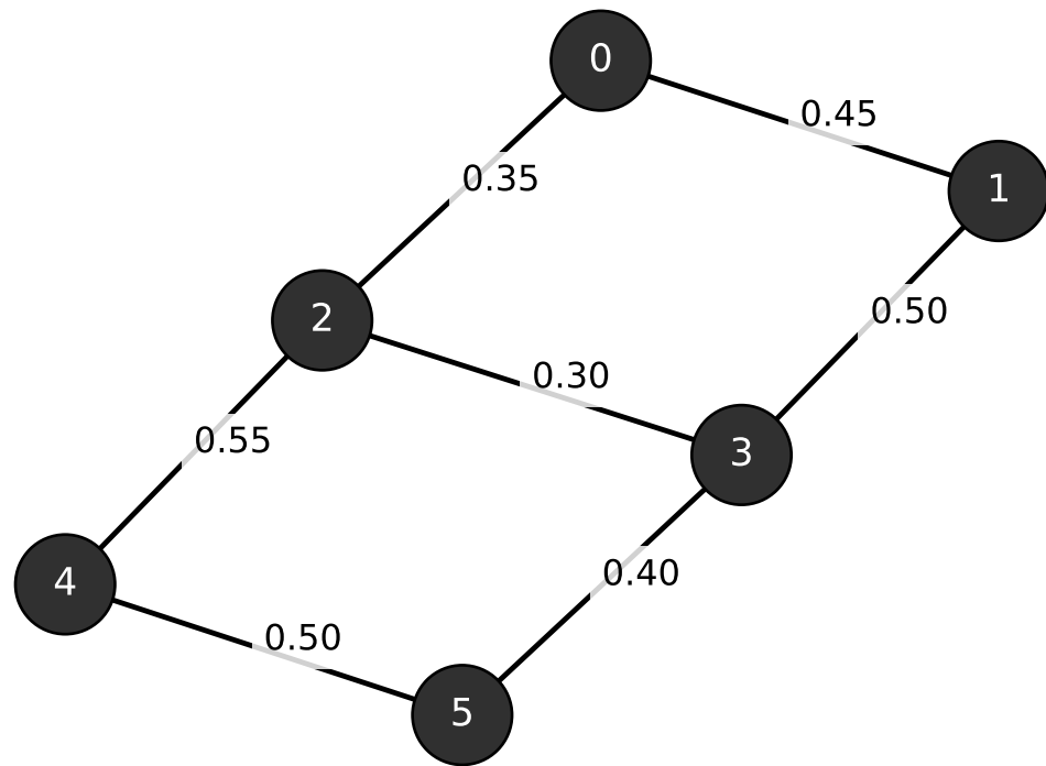
Independent-cascade network
