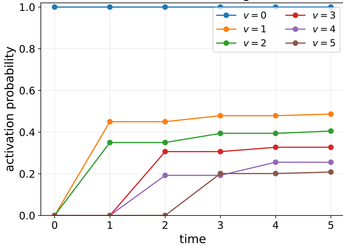
Exact activation marginals
