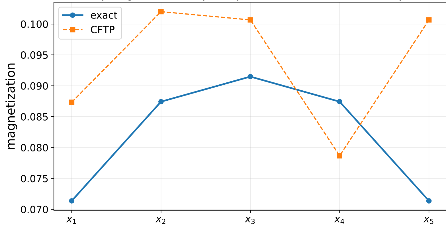
Coupling from the past produces unbiased samples
