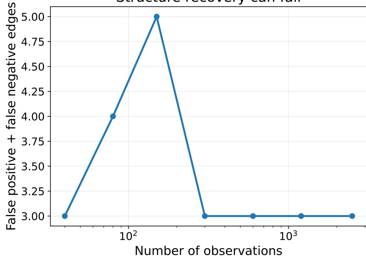
Structure recovery can fail
