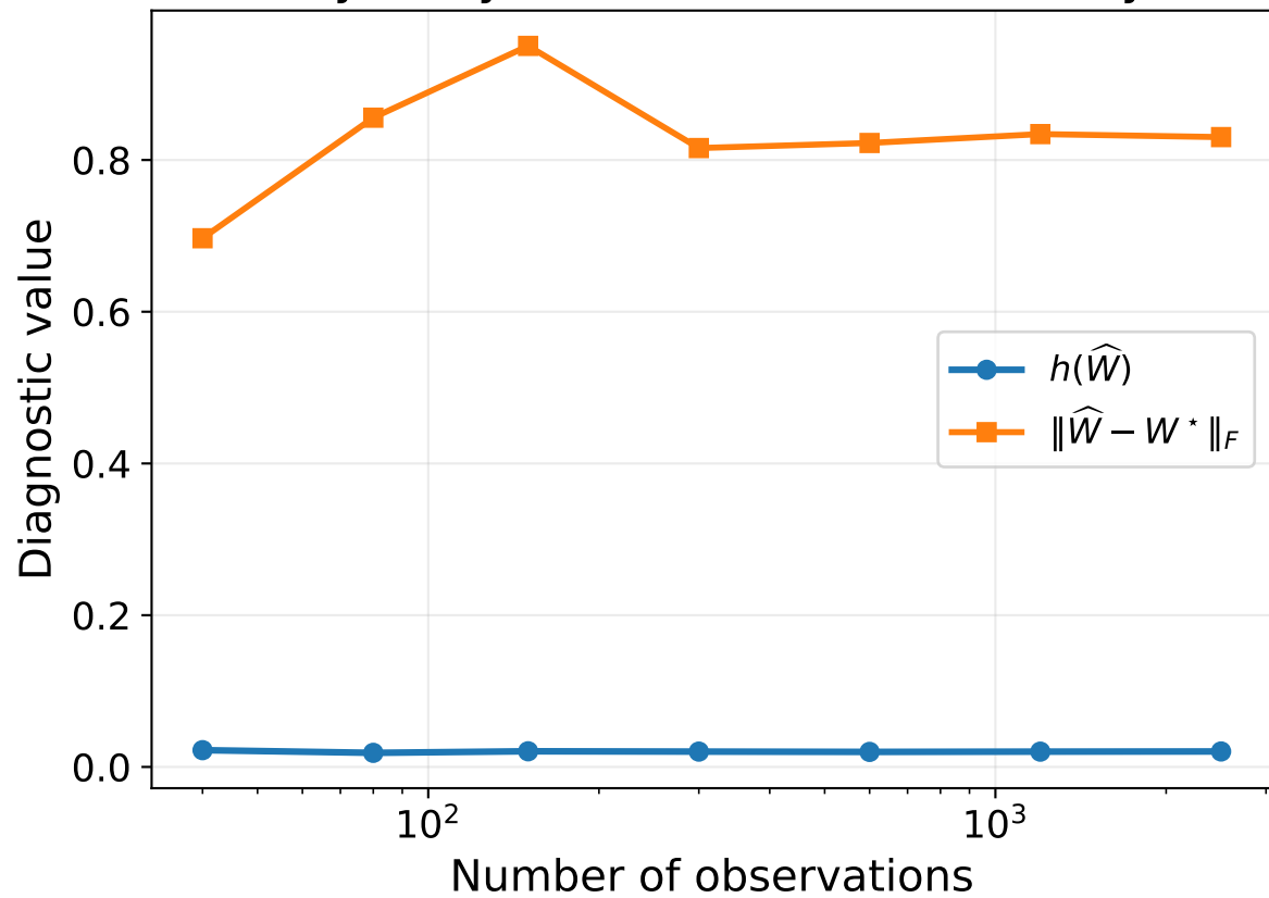
Acyclicity is not statistical accuracy
