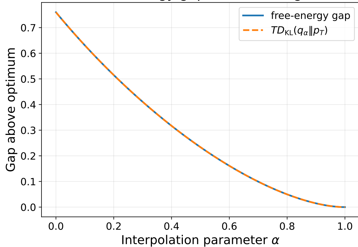
The free-energy gap is a KL divergence
