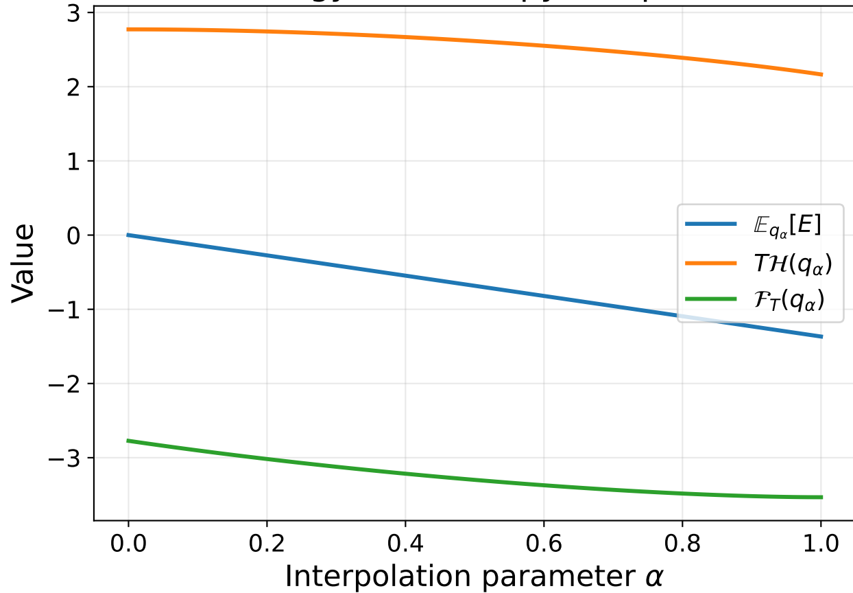
Energy and entropy compete
