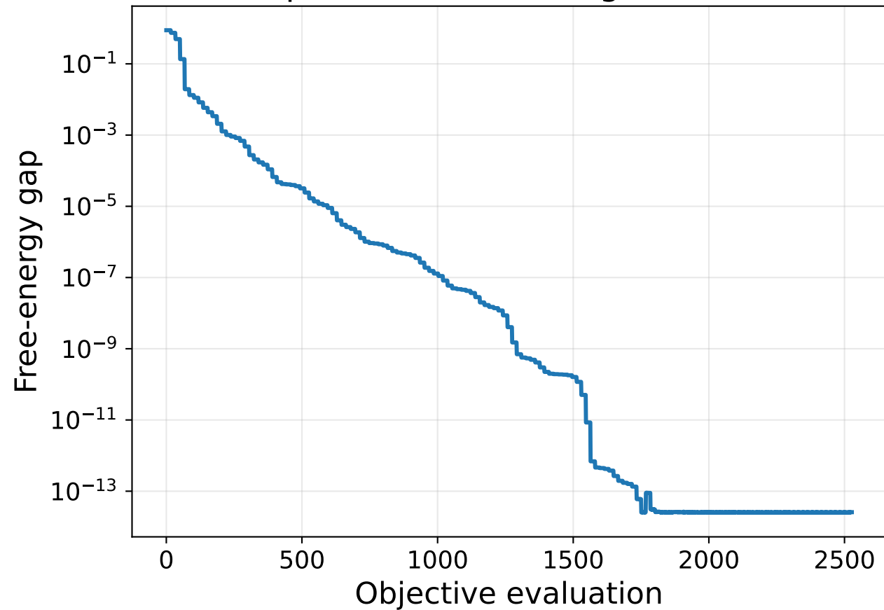
Variational optimization converges to the Gibbs law
