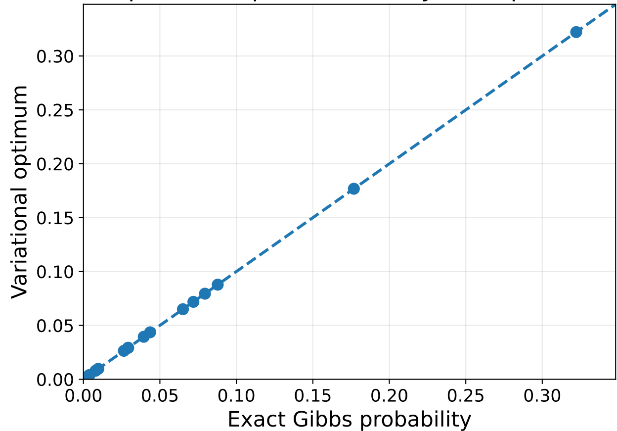
The optimum reproduces every state probability
