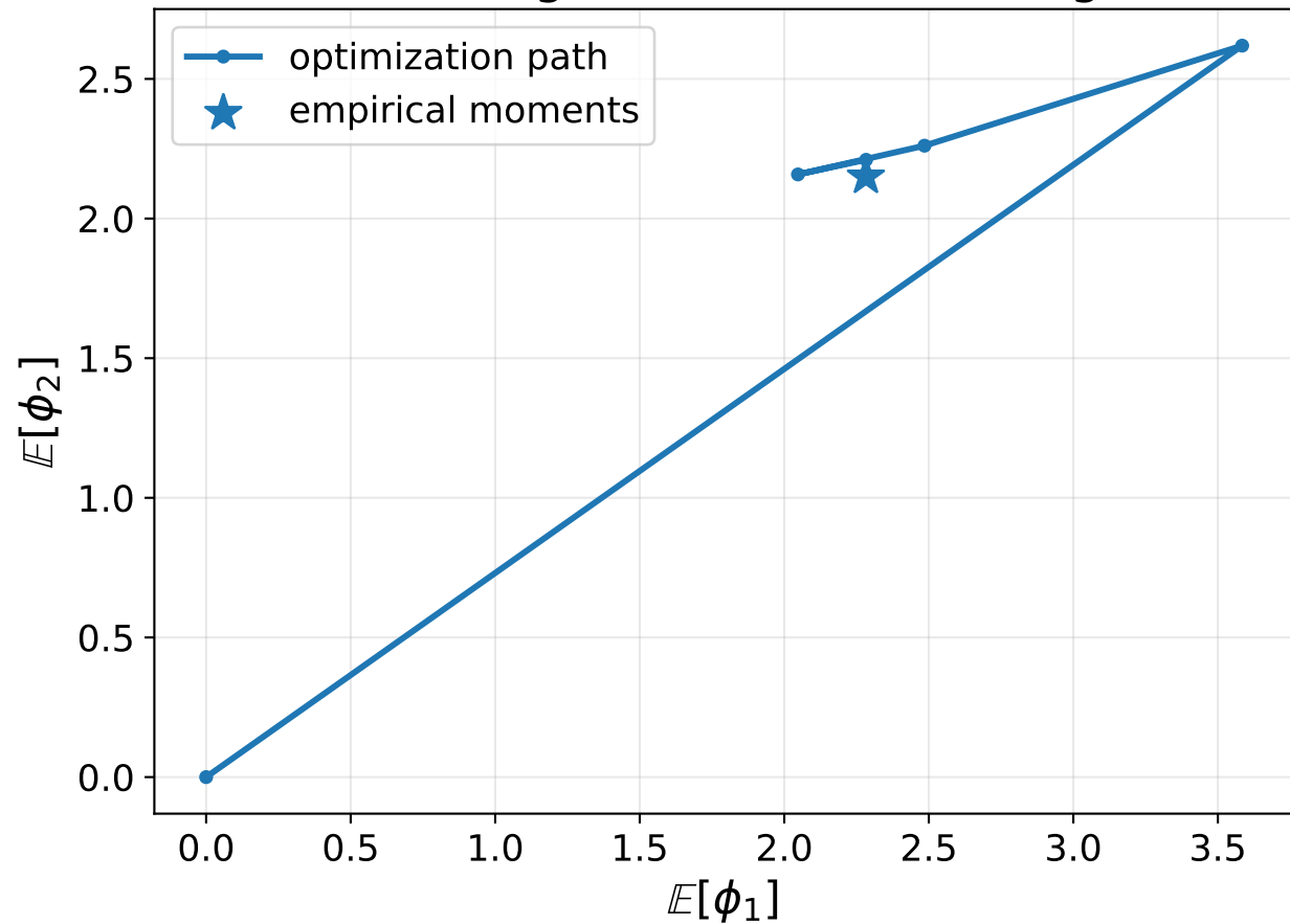
Learning is moment matching
