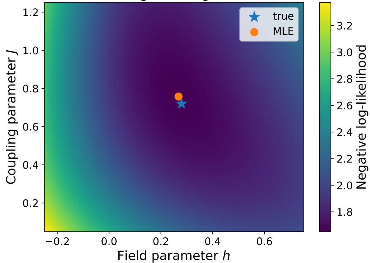
Convex negative log-likelihood
